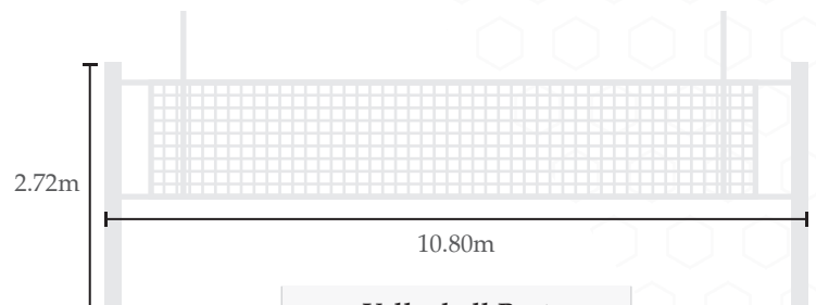
Volleyball Post TX-17 TX-25 TX-30
